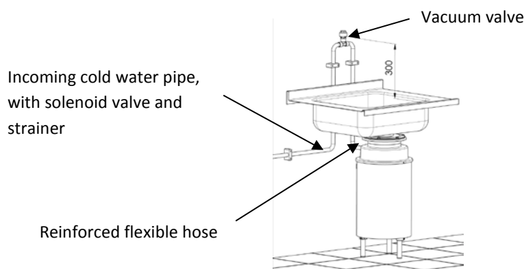
The picture above shows the positioning of a vacuum valve above a standard disposer sink assembly.
