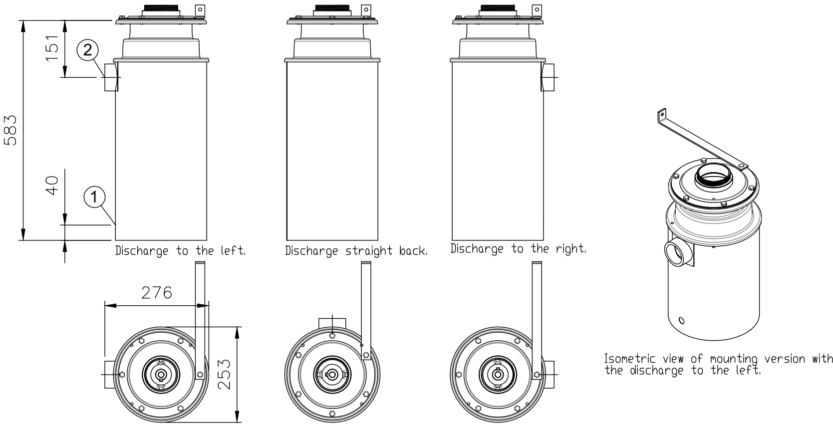
Installation principle side view
