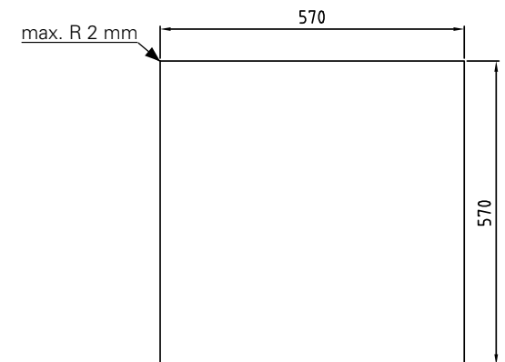
Dimensions of drop-in opening
