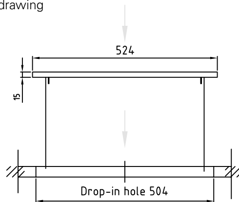
Mounting drawing
